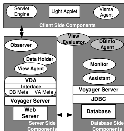
Figure 1: ViSMA Architecture
