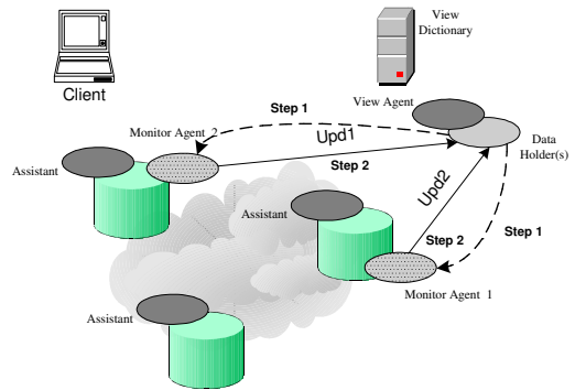
Figure 5: Datasource Monitoring
