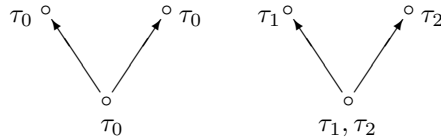
Figure 8. Satisfying (\tau_0 \neq \mathbf{0}) \wedge C(\tau_1, \tau_2) in a disjoint union of forks.
