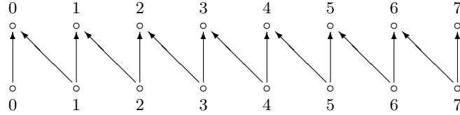
Figure 2. Satisfying the ‘counter formulas’ for n = 3 .
