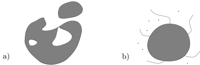
Figure 5. Shaded regions showing: a) a regular-closed subset of \mathbb{R}^2 , and b) a (closed but) not regular-closed subset of \mathbb{R}^2 .
