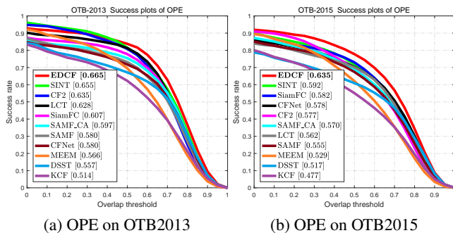
Figure 3: OPE Comparisons on OTB2013 (a) and OTB2015 (b).
