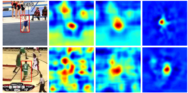
(a) ROI (b) SiamFC (c) EDSiam (d) EDCF Figure 1: Response maps learned by different methods for search instances ( gymnastics4 and basketball ). (a) Search instance, (b) Response map by SiamFC, (c) Response map by our Encoder-Decoder SiamFC (EDSiam), and (d) Response map by our Encoder-Decoder Correlation Filter (EDCF). EDSiam removes many noisy local minima in the response map of SiamFC. EDCF further refines the response map of EDSiam for more accurate tracking.
