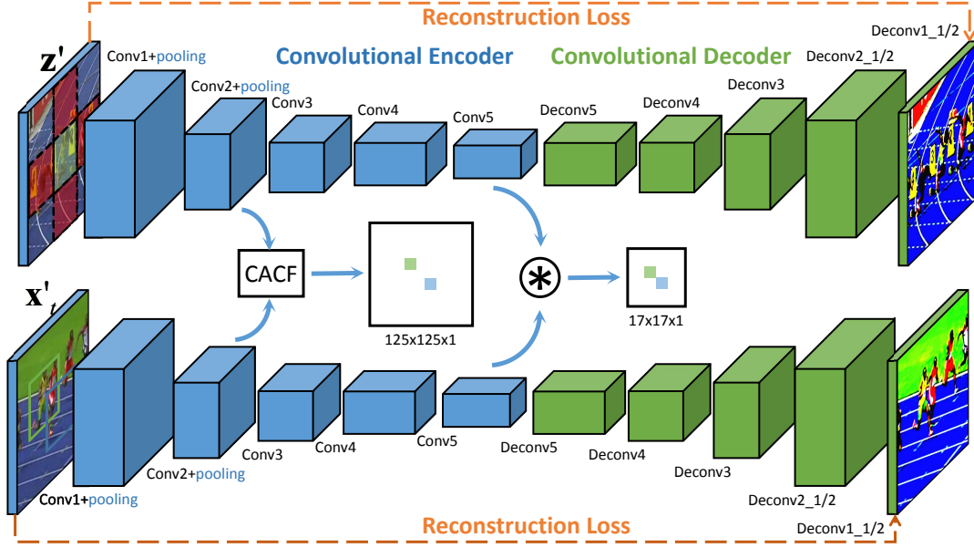
Figure 2: Architecture of EDCF, an Encoder-Decoder Correlation Filter . It consists of two fully convolutional encoder-decoder. Convolutional features are extracted from the initial exemplar patch \mathbf{z}' and the search patch \mathbf{x}'_t in frame t . The shallow features are exploited by the context-aware correlation filter tracker (CACF). The deep features that capture a high-level representation of the image are used in a cross correlation embedding without update online to avoid the drift problem. The reconstruction loss is used to enrich the detailed representation. Three hybrid loss is jointly trained in a mutual reinforced way.
